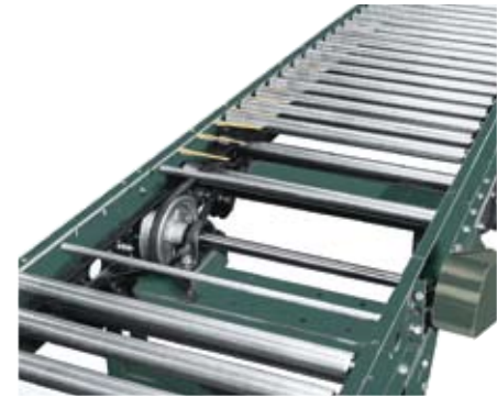
Conveyor sections are easily coupled together at either end to make up to 100 ft. long units. Drive is usually located near center of conveyor.
